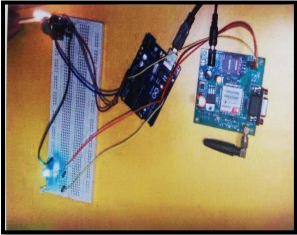
Smoke Detection and Sending Message using ARDUINO and GSM Module
