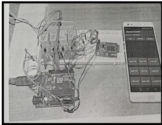
Bluetooth controlled fan / Light using ARUDINO and Relay module
